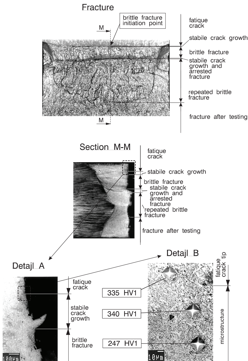
Figure 5: Fracture and microstructure in the vicinity of brittle fracture initiation point of specimen B \times B with surface crack ( a/W = 0.25 ) in the filler region of the homogeneous weld. At the vicinity of brittle fracture initiation point a bainitic microstructure (Detail ~ A) is visible, and at higher magnification (Detail - B) contours of primary ferrite (PF) can be seen, formed at primary \gamma grains [2].
