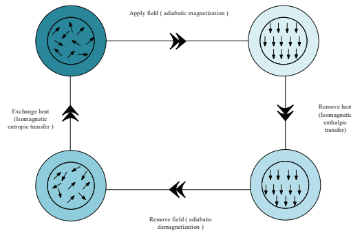
Figure 3: Thermodynamic processes in magnetic refrigeration
